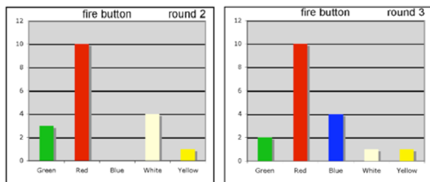
Figure 9. Choice for fire button in rounds 2 and 3.
