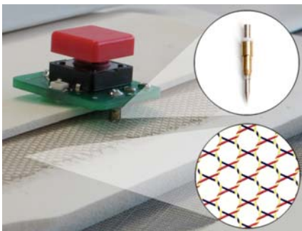
Figure 2. VoodooPin Button control with Pin&Play connector, and cross-section of Pin&Play substrate fabric revealing internal network layers.
